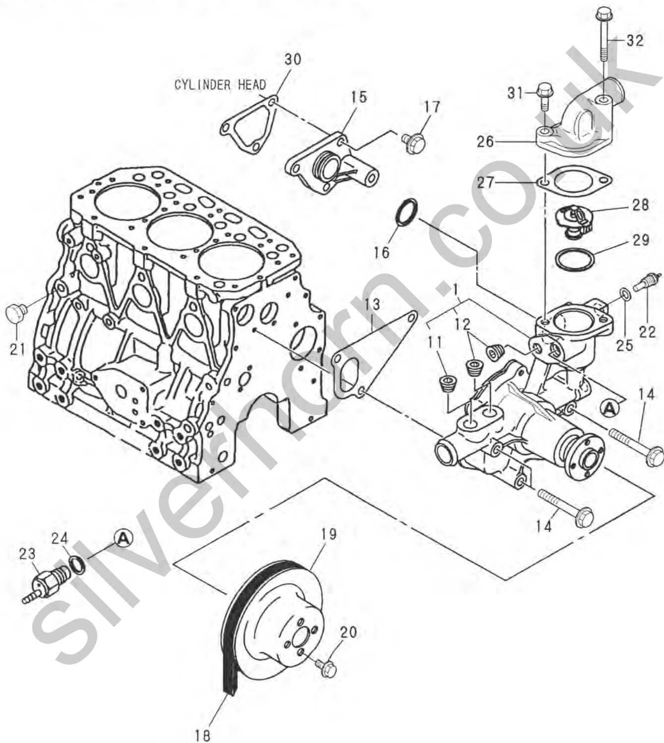
Fig. 10 COOLING WATER SYSTEM
