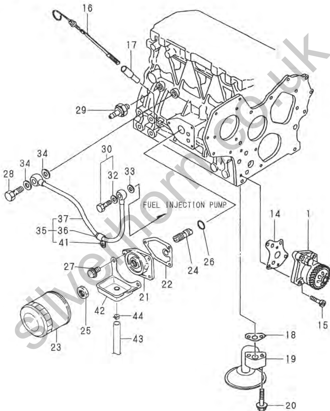
Fig. 9 LUB. OIL SYSTEM
