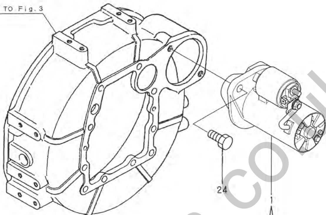
Fig. 15 STARTING MOTOR
