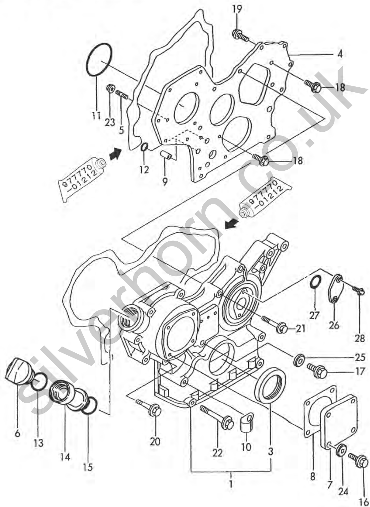
Fig. 2 GEAR HOUSING
