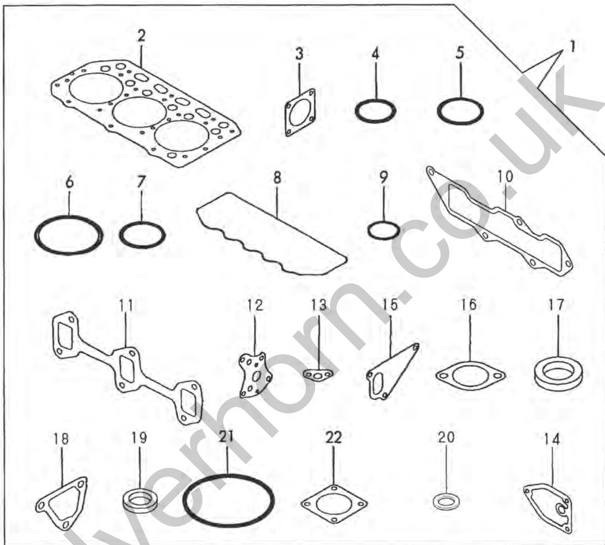
Fig. 17 GASKET SET (OPTIONAL) & TOOLS
