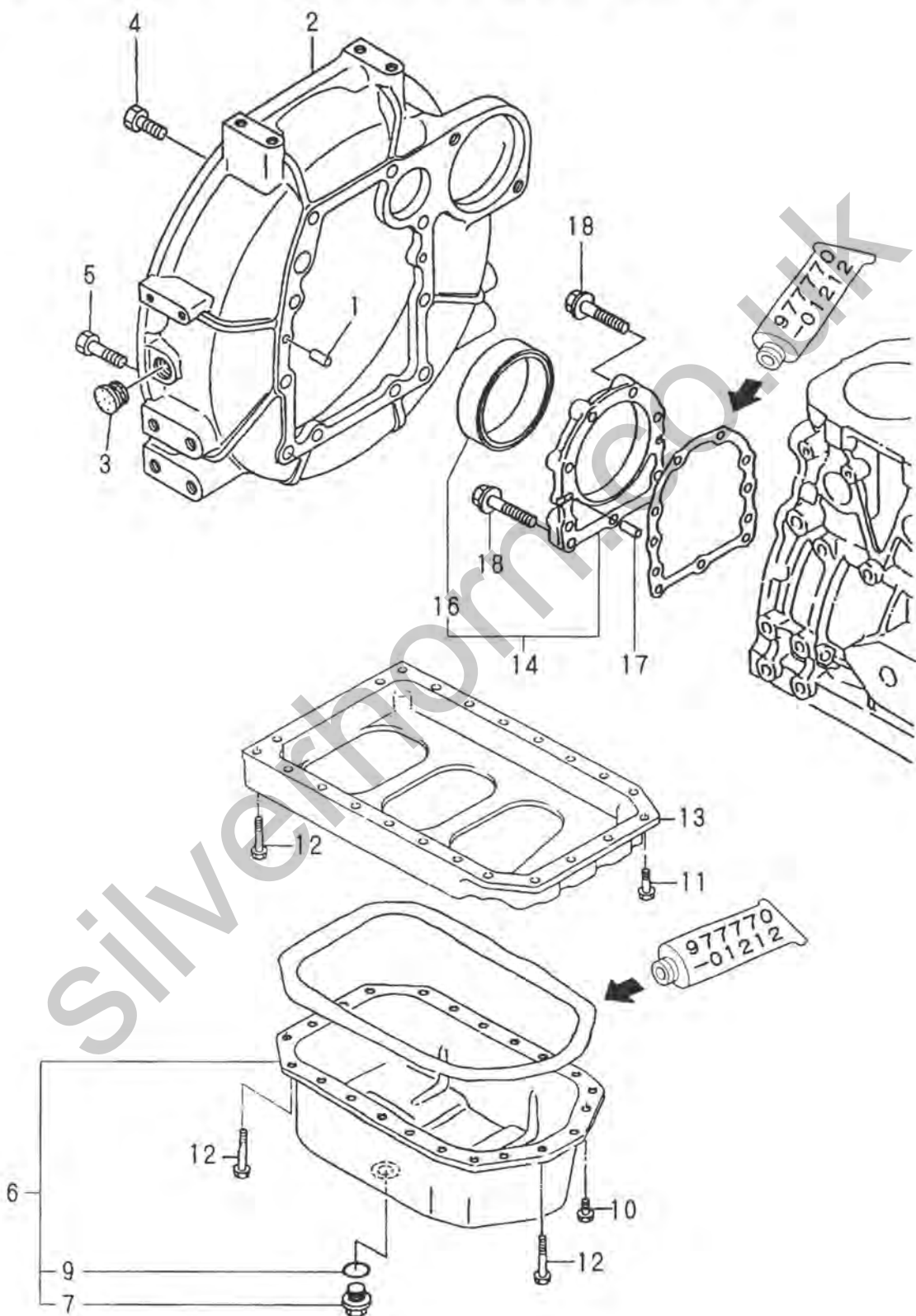
Fig. 3 FLYWHEEL HOUSING & LUB. OIL SUMP
