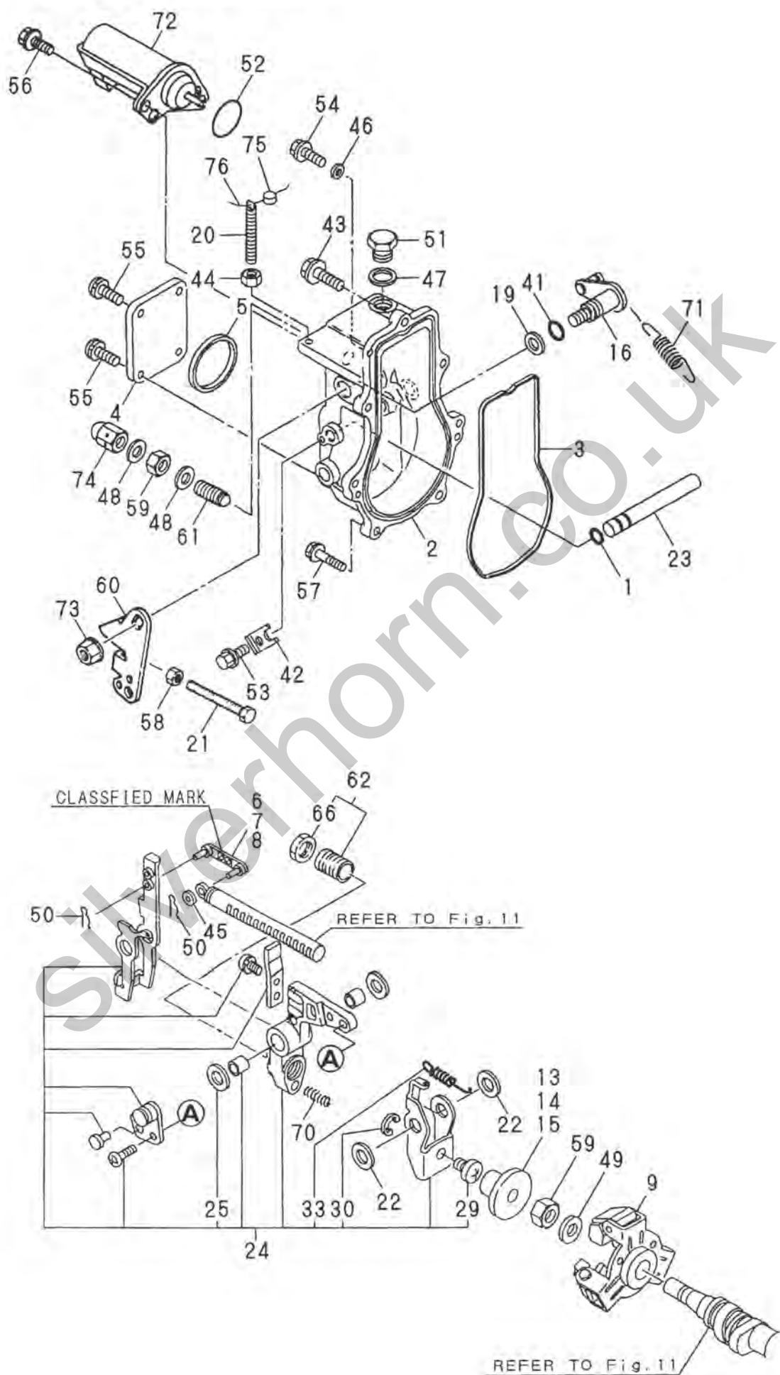
Fig. 12 GOVERNOR
