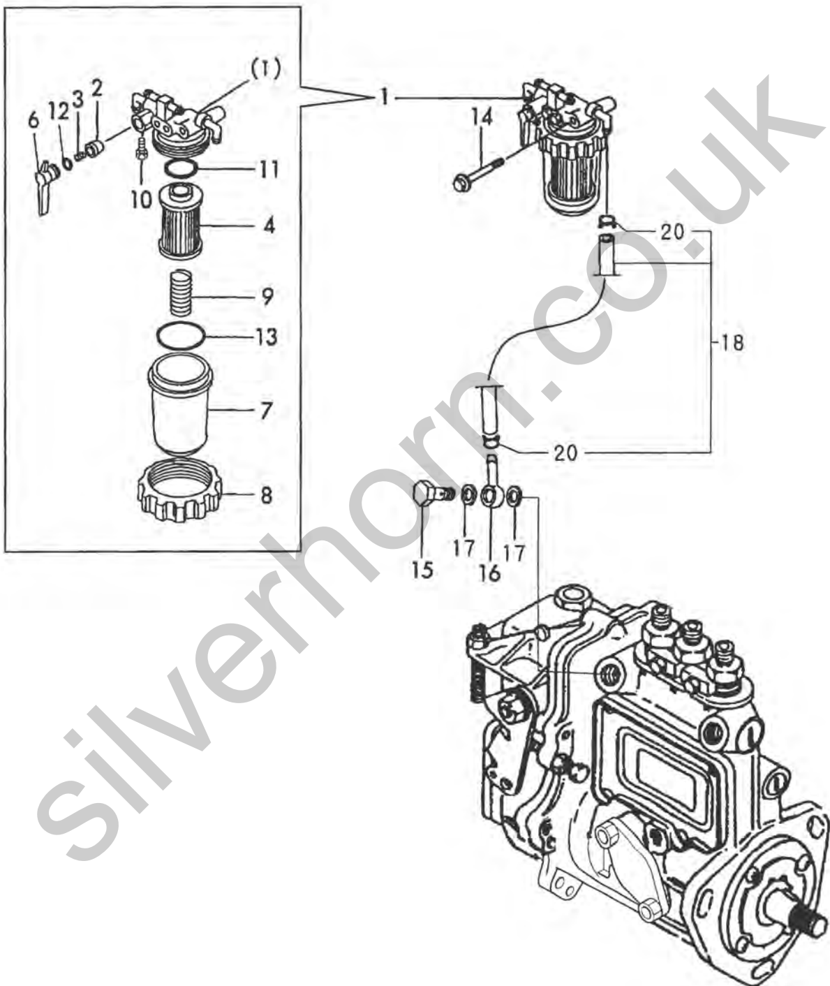
Fig. 14 FUEL PIPE
