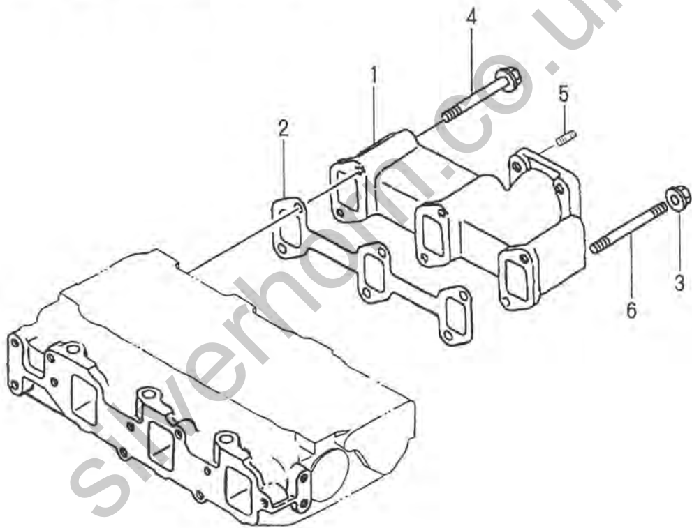
Fig. 6 EXH. MANIFOLD
