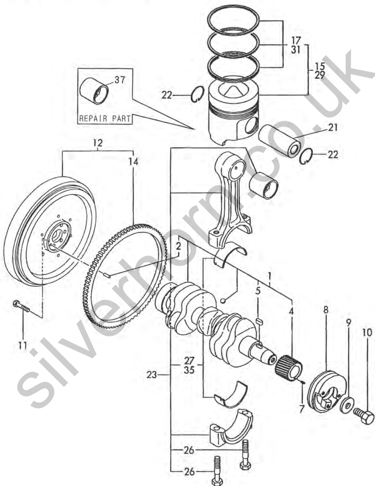
Fig. 8 CRANKSHAFT & PISTON
